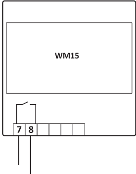
Fig. 14 Digital output
