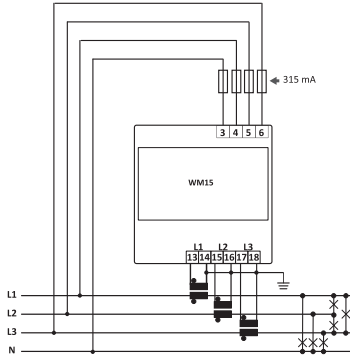
Fig. 11 Three-phase with neutral (4-wire)
