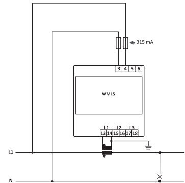
Fig. 10 Single-phase (2-wire)
