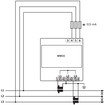
Fig. 12 Three-phase without neutral (3-wire) - ARON
