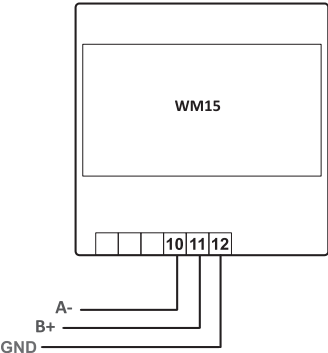
Fig. 15 RS485 port
